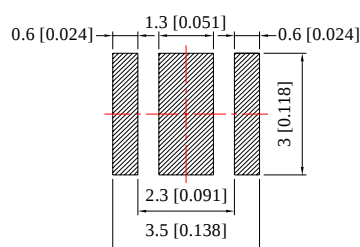
Recommended Soldering Pad Dimensions
