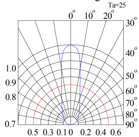
Radiation Diagram
