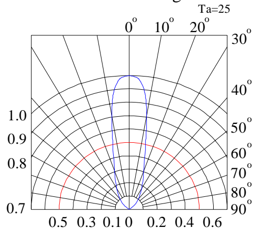
Radiation Diagram
