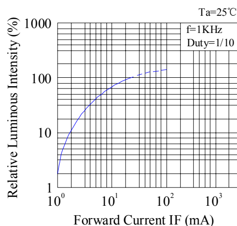
Luminous Intensity & Forward Current Ta=25°C f=1KHz Duty=1/10
