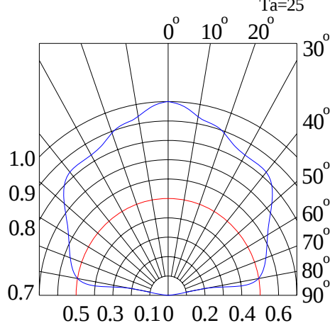
Radiation Diagram
