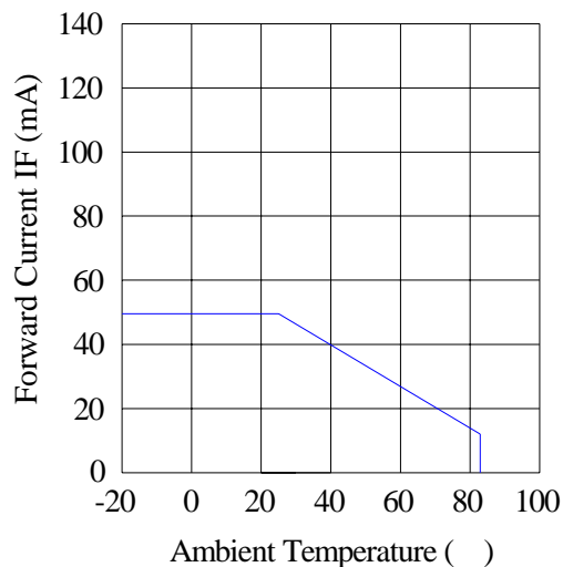
Forward Current & Ambient Temperature
