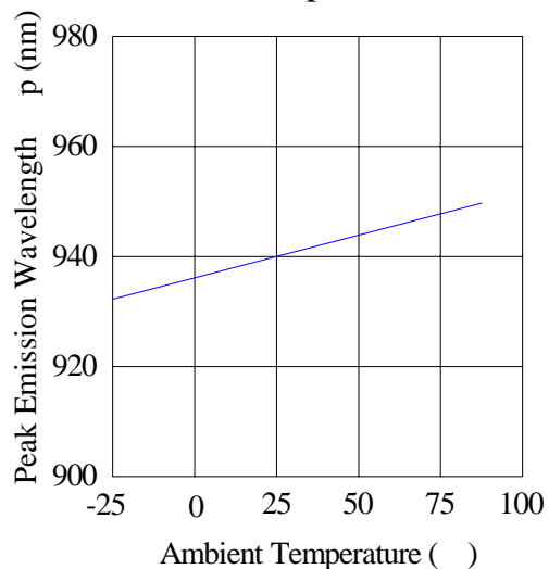
Peak Emission Wavelength & Ambient Temperature
