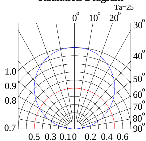
Radiation Diagram
