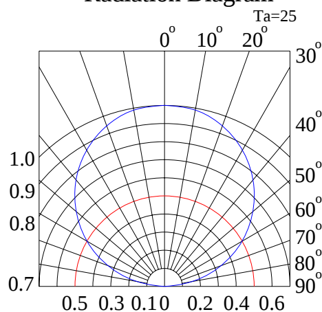
Radiation Diagram
