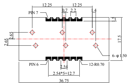
Recommended Soldering Pad Dimensions
