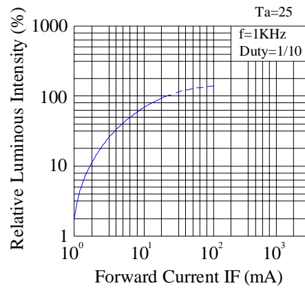
Luminous Intensity & Forward Current T_a=25
