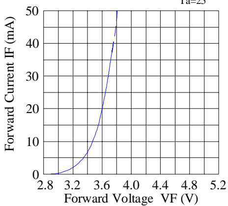
Forward Current & Forward Voltage T_a=25
