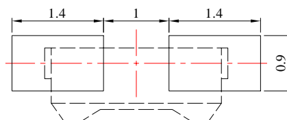
Recommended Soldering Pad Dimensions
