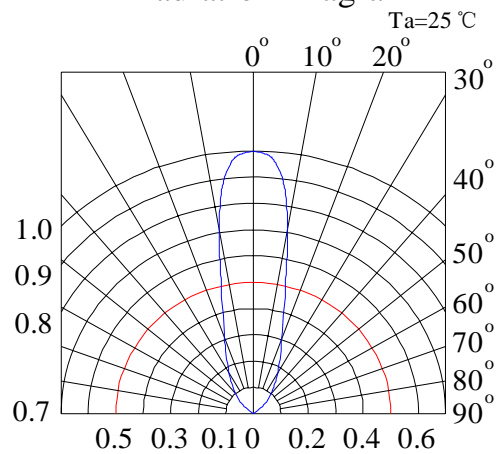
Radiation Diagram
